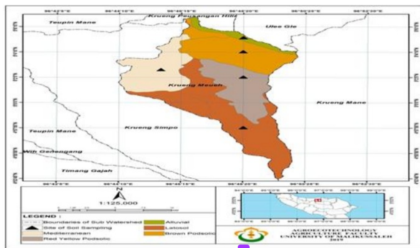
Figure 1: Map of soil types in the study area
