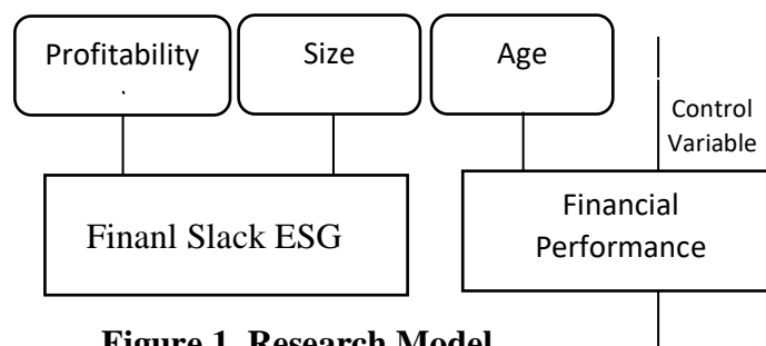
Figure 1. Research Model
