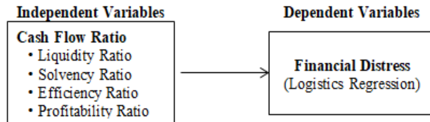
Figure 1. Framework
