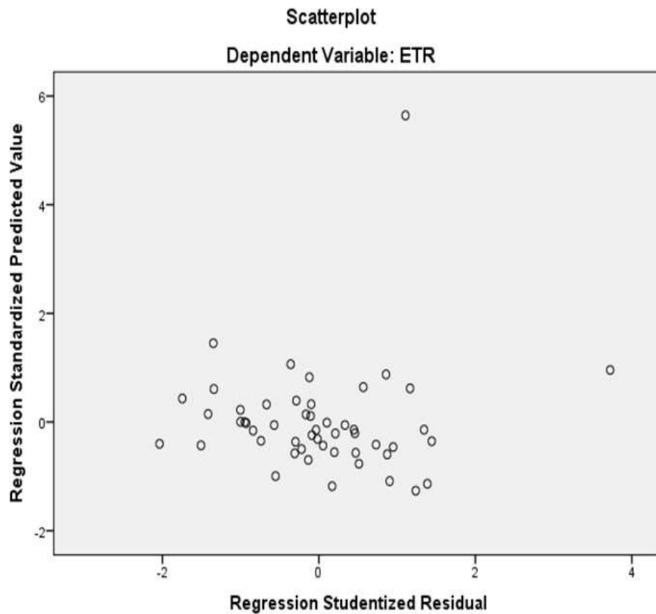
Figure 2. Scatterplots
