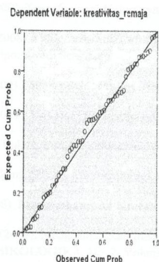
Gambar 1 Normal PP Plot
