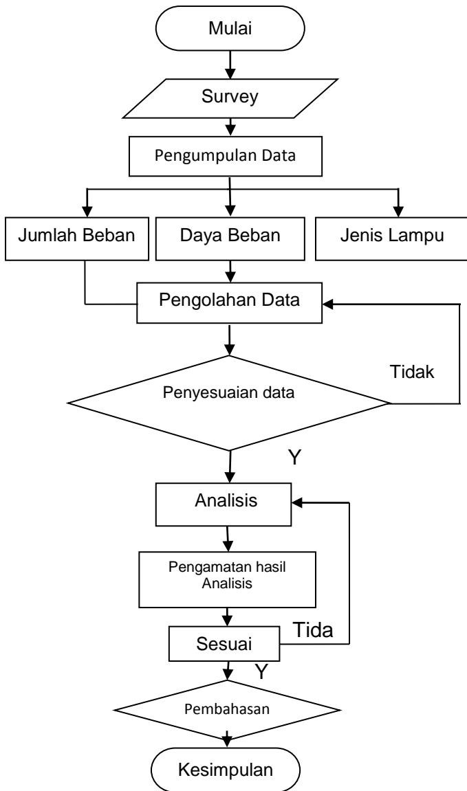
Gambar 3.1 Flowchart
