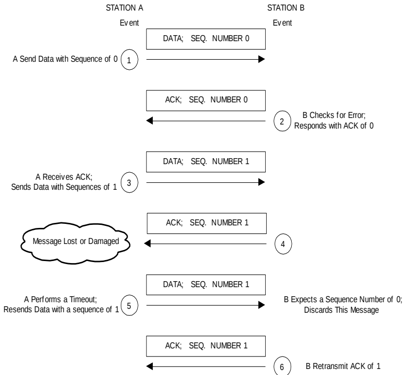
Gambar 3.7 Stop-and-wait alternating sequence
