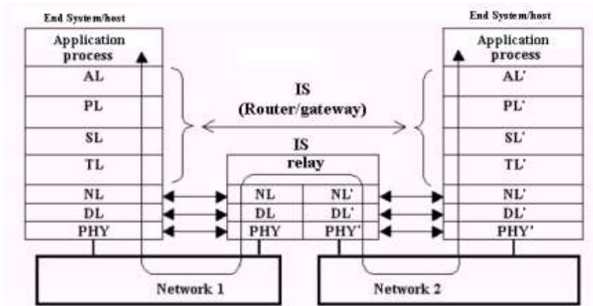
Gambar 4.13 Router /gateway
