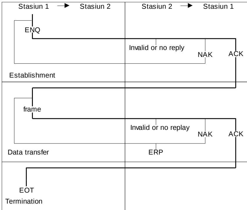
Gambar 3.3 Hubungan kendali point-to-point
