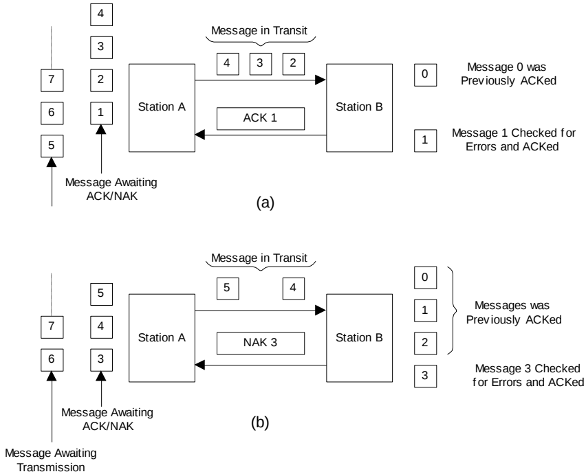
Gambar 3.8. Sliding window data link control
