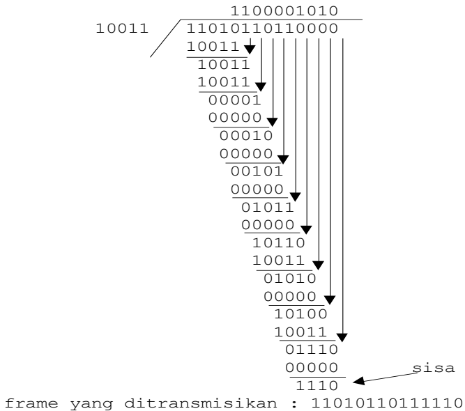
Gambar 3-12. Perhitungan checksum kode polynomial
