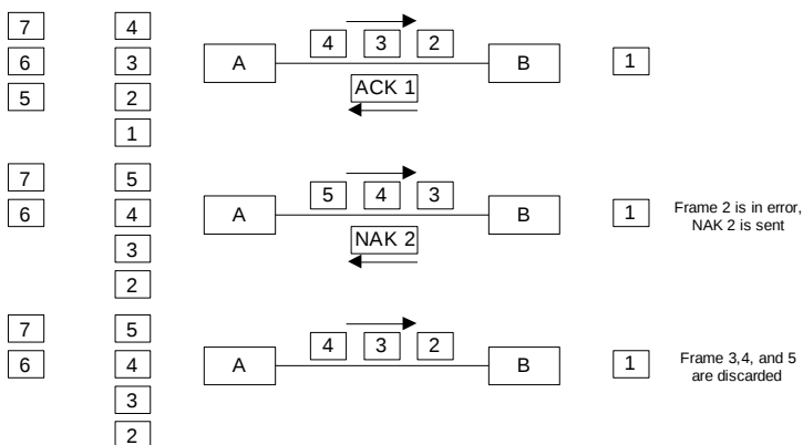
Gambar 3.14 Go-back-N ARQ
