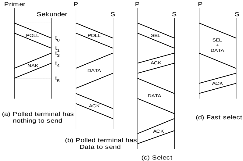
Gambar 3.4 Poll and select sequences
