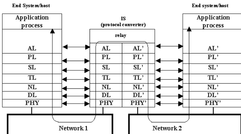
Gambar 4.14 Protocol converter
