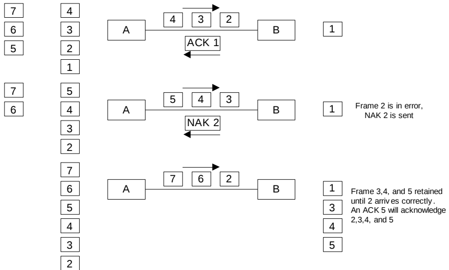
Gambar 3.14 Selective-report ARQ
