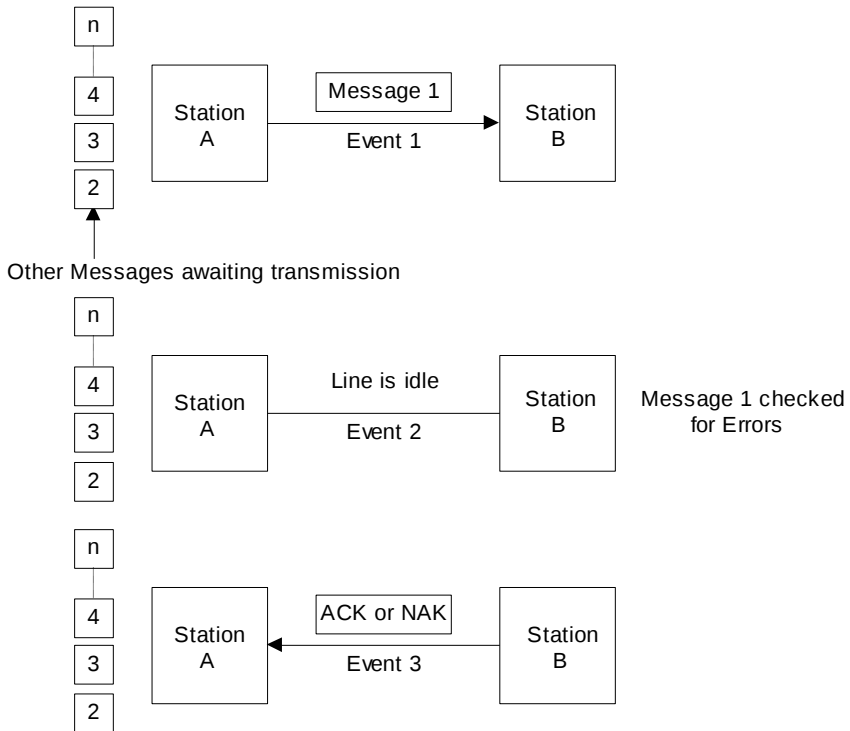
Gambar 3.6 Stop and wait data link control
